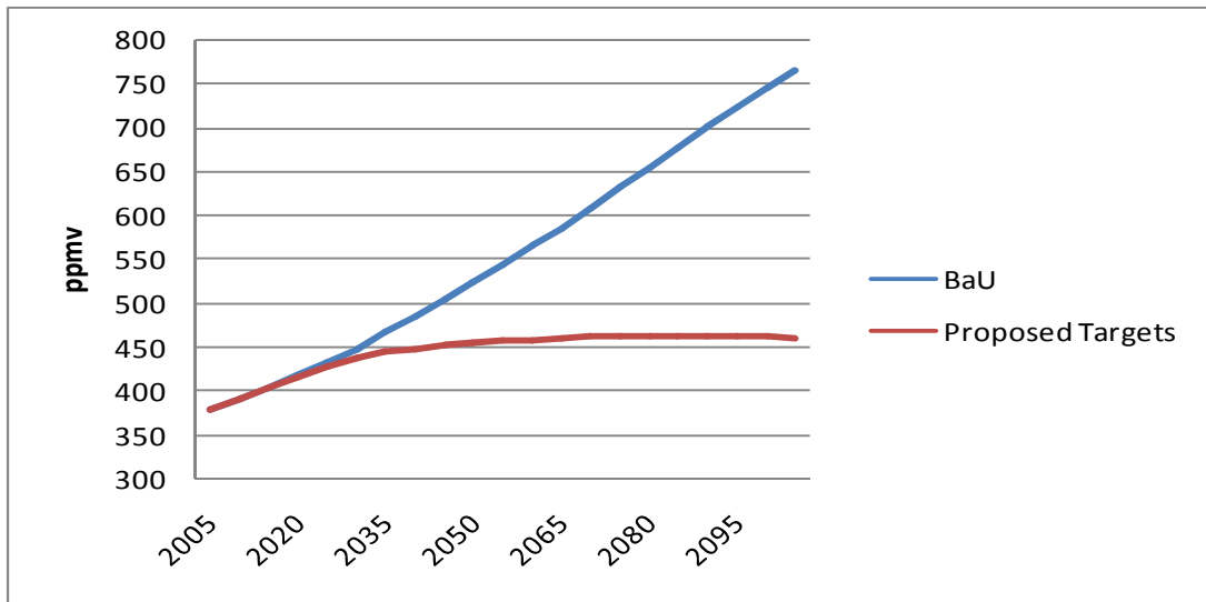
Figure 10: CO 2 concentrations achieve year-2100 concentration goal of 460 ppm
