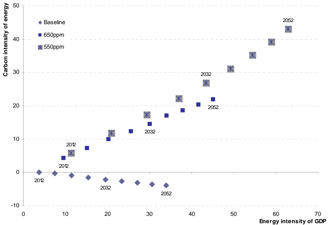
Figure 2. World energy intensity and carbon intensity trajectories under alternative carbon price paths
