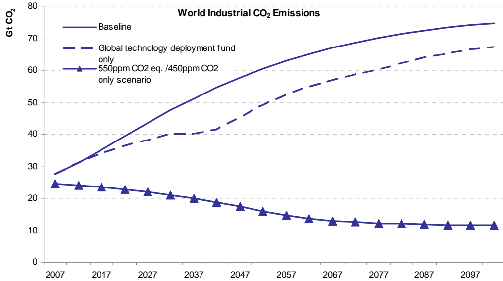
Figure 22. Projected CO 2 emissions and concentration under a global technology deployment policy only
