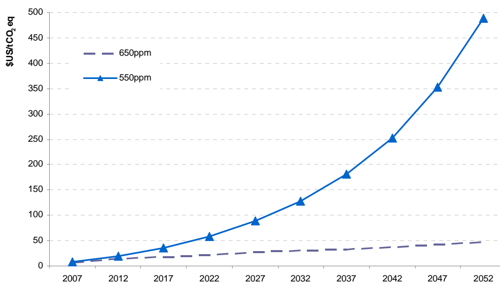
Figure 1. Carbon price paths under 550 ppm and 650 ppm GHG concentration scenarios
