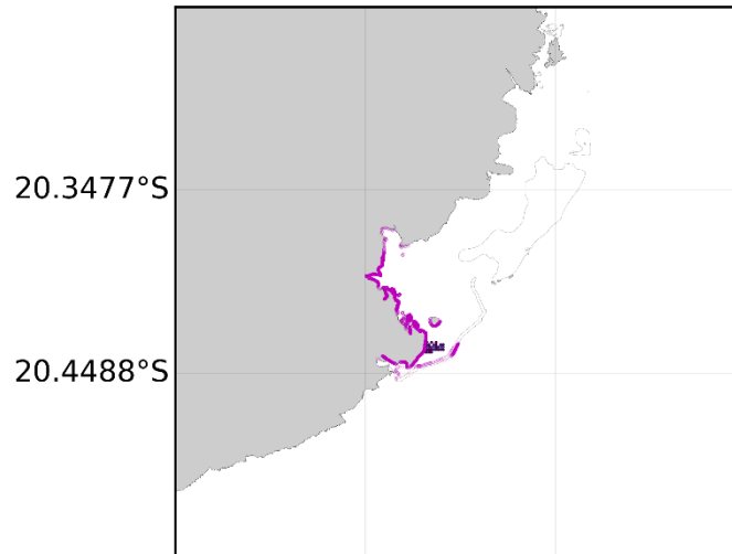
Surface oil concentration (colorscale) and beached oil (in purple) on the 21/08/2020 03:00
