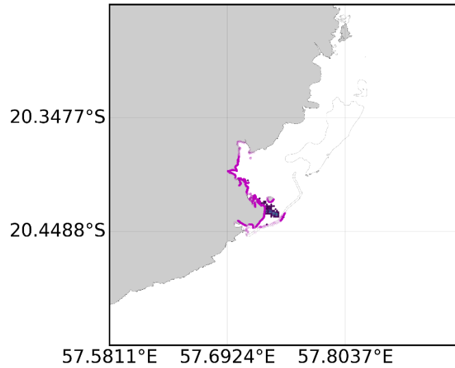
Surface oil concentration (colorscale) and beached oil (in purple) on the 22/08/2020 23:00
