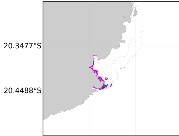
Surface oil concentration (colorscale) and beached oil (in purple) on the 20/08/2020 03:00
