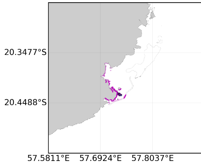
Surface oil concentration (colorscale) and beached oil (in purple) on the 23/08/2020 23:00
