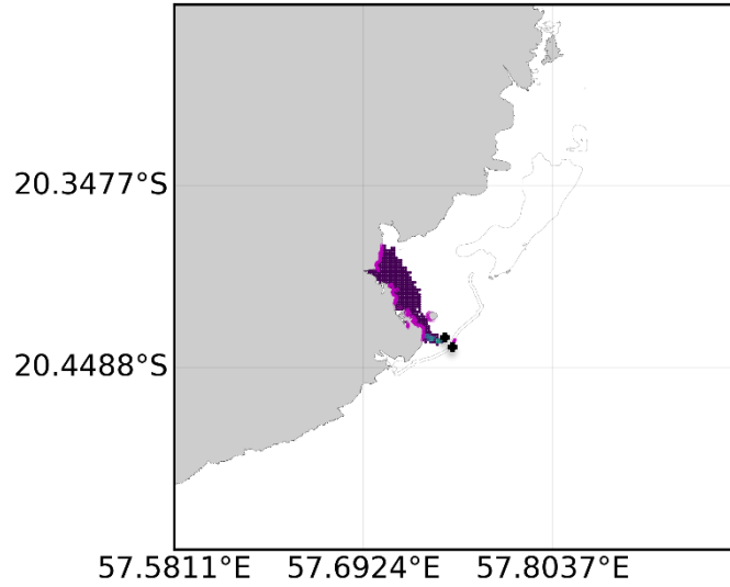
Oil spill initial condition (10/08/2020 03:00). Black crosses mark spill origins.
