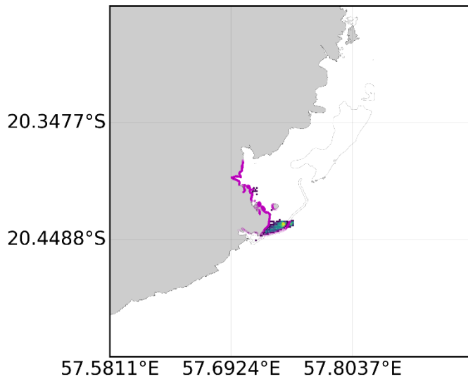
Surface oil concentration (colorscale) and beached oil (in purple) on the 11/08/2020 03:00
