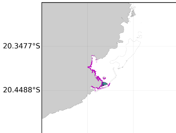
Surface oil concentration (colorscale) and beached oil (in purple) on the 20/08/2020 03:00
