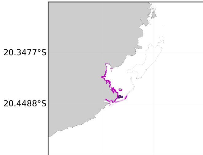
Surface oil concentration (colorscale) and beached oil (in purple) on the 21/08/2020 03:00
