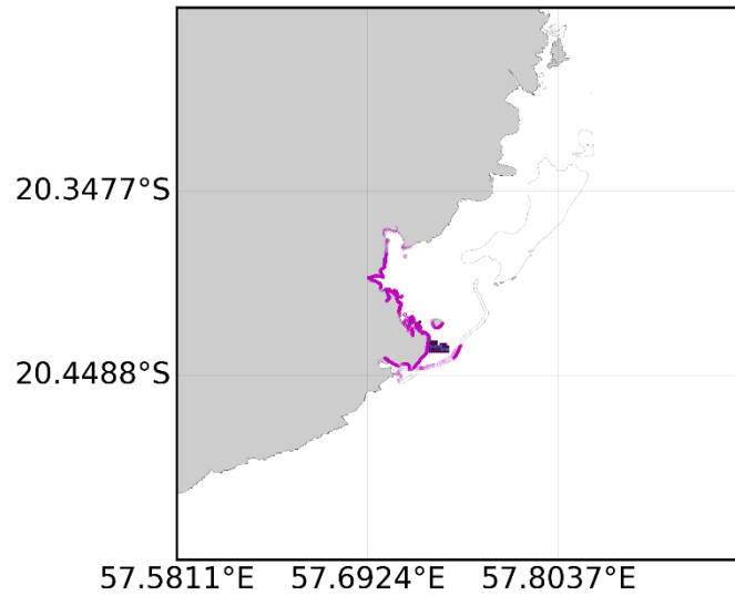
Surface oil concentration (colorscale) and beached oil (in purple) on the 22/08/2020 12:00
