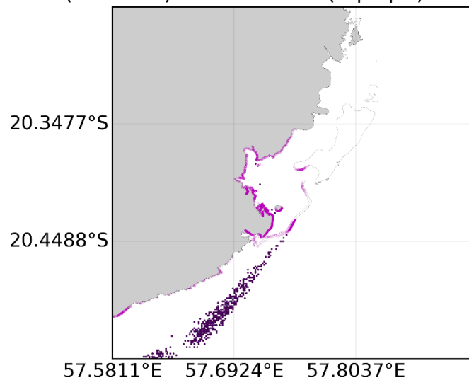
Surface oil concentration (colorscale) and beached oil (in purple) on the 30/08/2020 12:00
